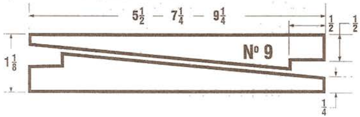
5/4 BEVEL SIDING; SHIPLAP JOINT
