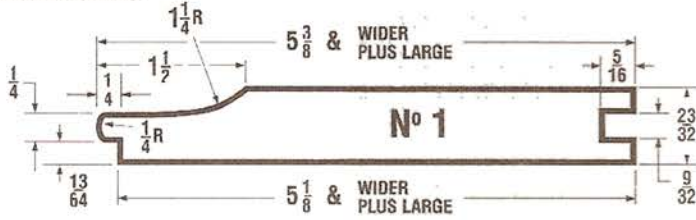
COVE SIDING
