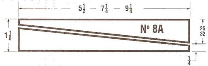
5/4 BEVEL SIDING
