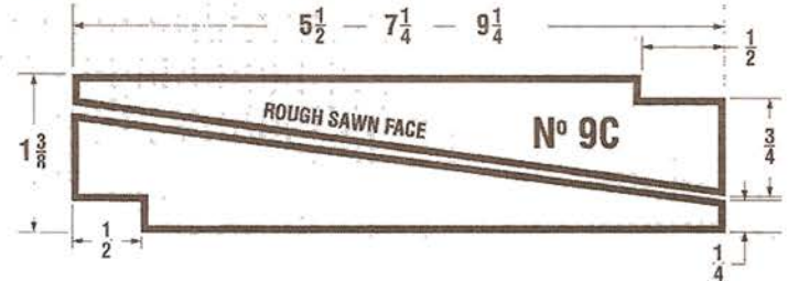
6/4 BEVEL SIDING; SHIPLAP JOINT
