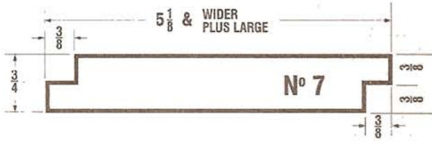
SHIPLAP SIDING
